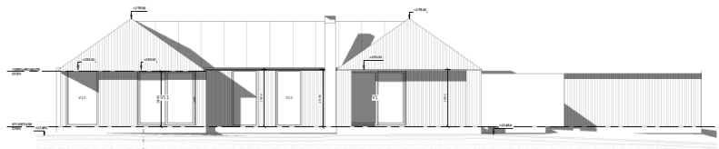
FACADE MOD VEST 1 : 50
