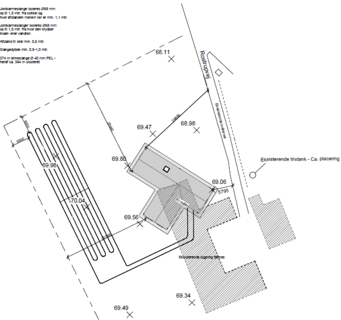
Situationsplan
