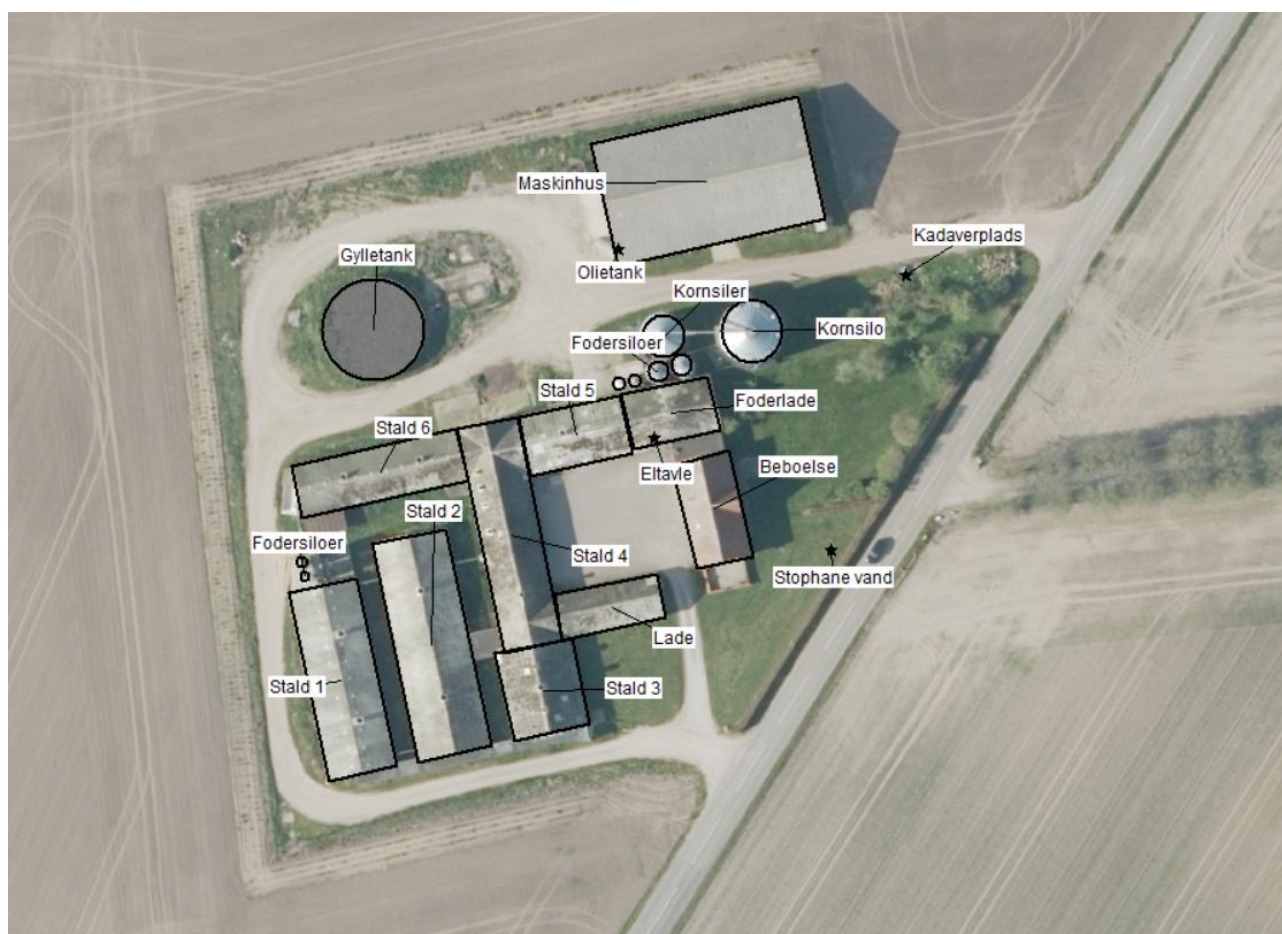
Situationsplan
