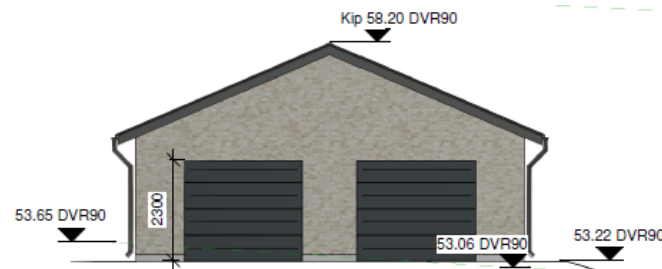
Facade vest
