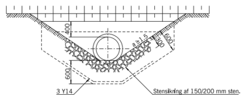
SNIT B - B
