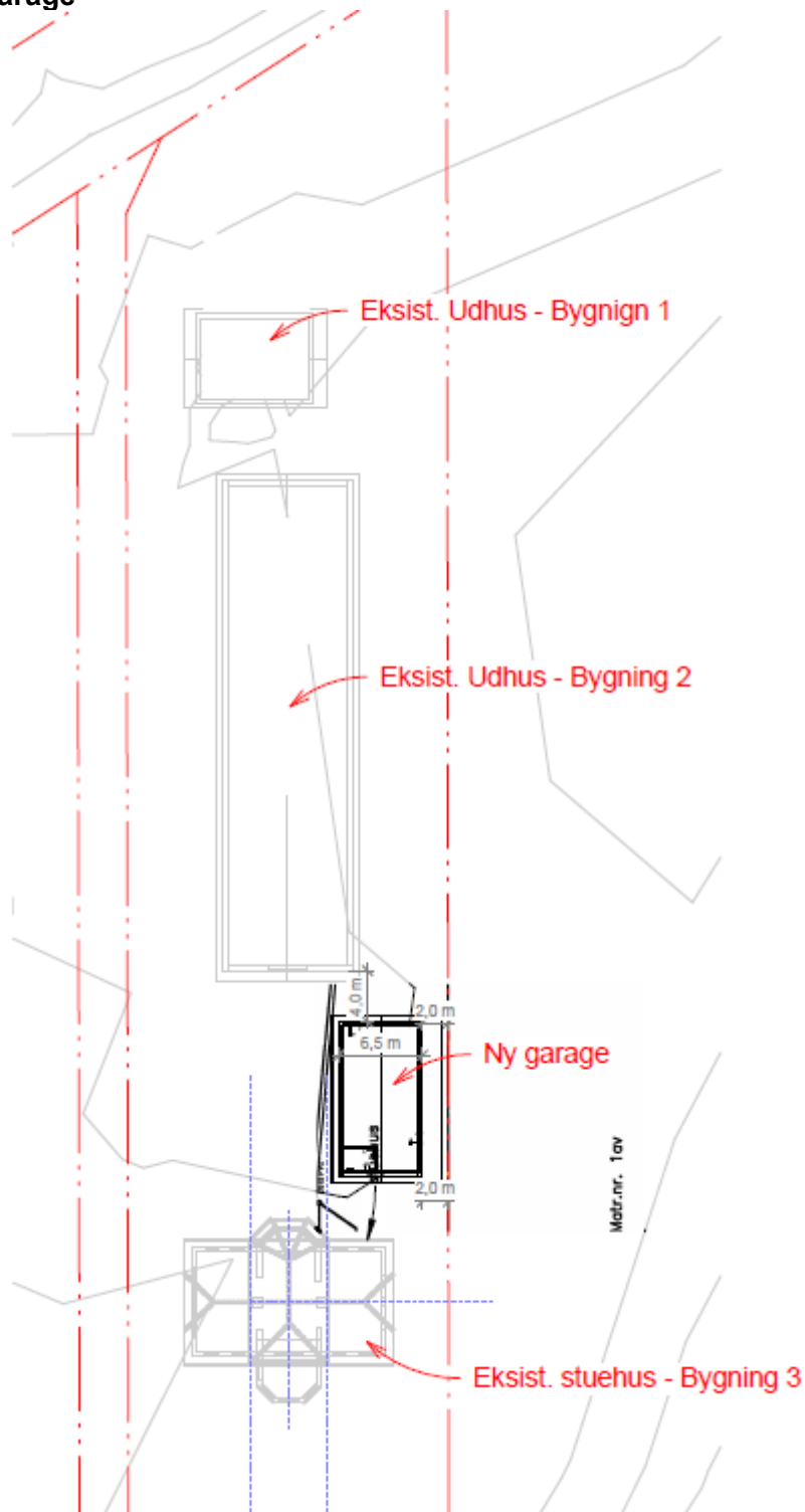
Figur 1: Situationstegning for garagen
