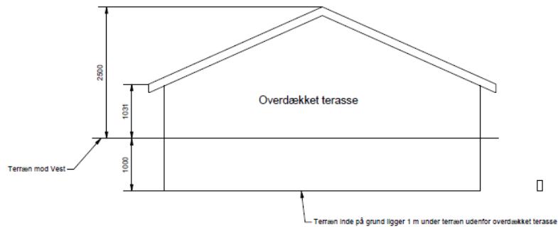
Facade vest
