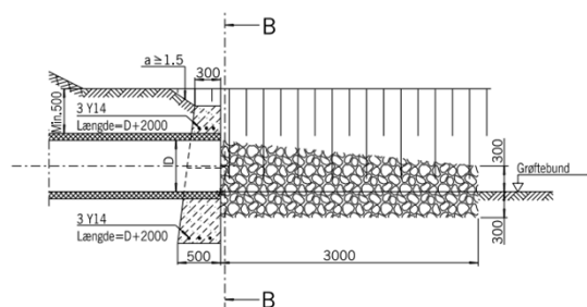
SNIT A - A
